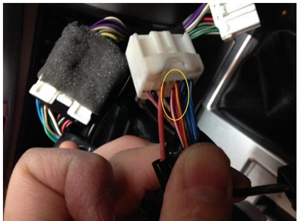
14 PIN Version
